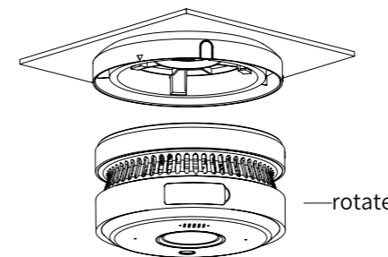
Figure 3-4 Installation (3)
