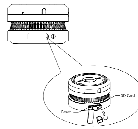
Figure 3-6 SD Card
