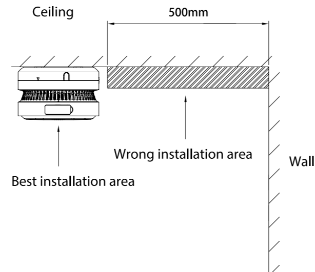
Figure 3-1 Installation position
