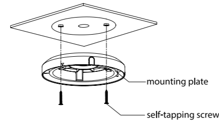
Figure 3-3 Installation (2)
