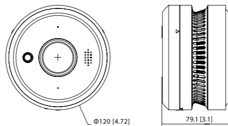
Figure 1-1 Dimensions (mm[inch])
