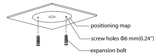
Figure 3-2 Installation (1)
