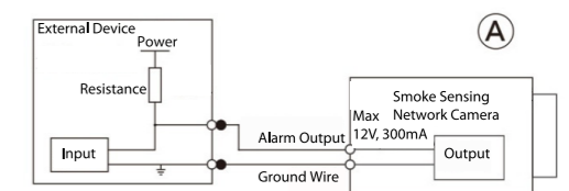
Figure 1-4 Alarm output
